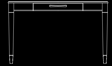
3730-113 DESK with DRAWER inches: 48w 28d 30h centimeters: 122w 71d 76h
