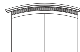
3553-230 HEADBOARD/FOOTBOARD inches: 39w 2d 24h (39w 1d 18h) centimeters: 99.5w 5.5d 61h (99.5w 3d 46h)
