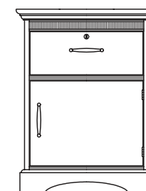
3553-728 BEDSIDE CABINET inches: 22w 19d 30h centimeters: 56w 48.5d 76.5h
