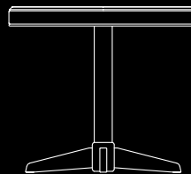
3560-324 ROUND TOP GUEST TABLE inches: 34dia 30h centimeters: 86.5dia 76.5h
