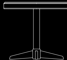
3779-324 ROUND TOP GUEST TABLE inches: 34dia 30h centimeters: 86.5dia 76.5h
