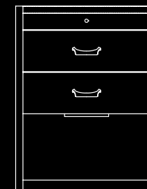
3775-050 NIGHT STAND inches: 24w 19d 32h centimeters: 61w 48.5d 81.5h
