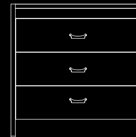
3775-040 CHEST inches: 38w 20d 38h centimeters: 97w 51d 97h
